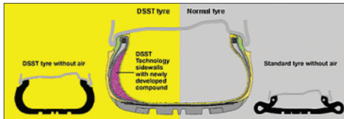
Typical Construction of run flat tyre and comparison to standard tyre when flat.
